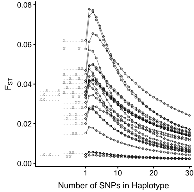
Figure S4. F_{ST} as a function of the number of SNPs in windows of neighboring SNPs, for pairs of geographic regions. Each of 21 pairs of regions is considered. Each point indicates the median of 10,000 F_{ST} values, one for each of the 10,000 windows. Each pair of regions is indicated by a pattern of “.” and “X” symbols, with X indicating that a region is included. The left-to-right order of regions is Africa, Middle East, Europe, Central/South Asia, East Asia, Oceania, America. Thus, for example, .X...X. indicates the pair (Middle East, Oceania).
