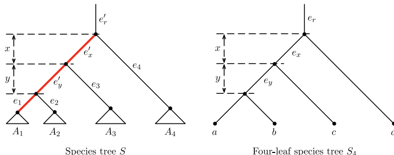
FIG. 4. A tree with at least five leaves ( left ), illustrating the embedded structure of an asymmetric four-leaf tree ( right ). The path with length at least three between the root and some leaf is shown with a thick line. Each of the triangles, representing taxon groups, contains at least one leaf.
