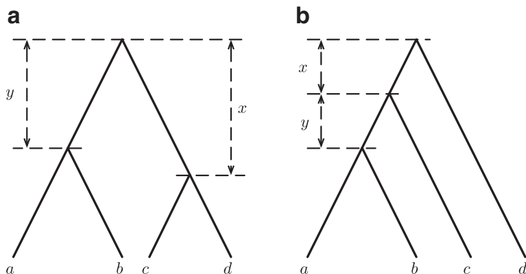
FIG. 2. Symmetric (a) and asymmetric (b) rooted, binary trees with leaf labels a, b, c, and d.
