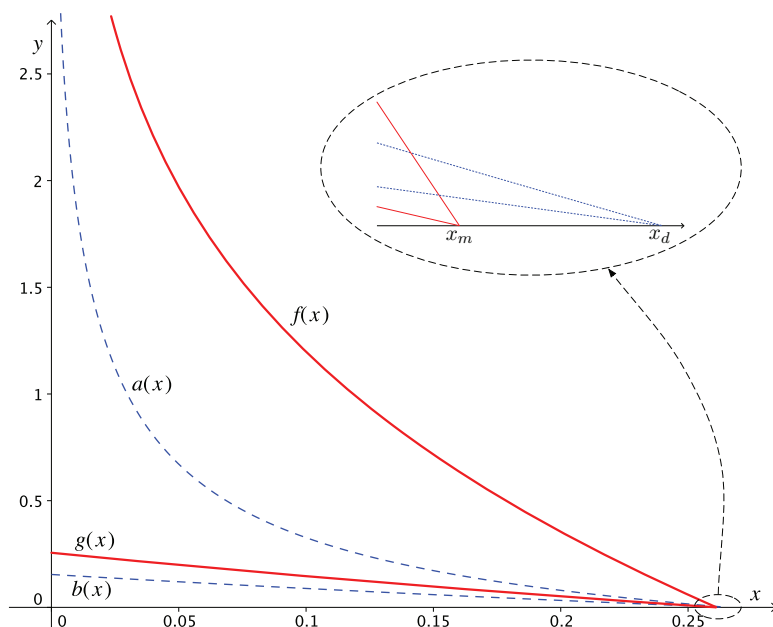
FIG. 3. Anomaly zones of the minimizing-deep-coalescence (MDC) criterion for asymmetric species trees with four leaves. In the region bounded by y = g(x) and the two axes, there are three candidate species trees with lower expected deep coalescence costs than the true species tree, while in the region bounded by the y -axis, y = g(x) and y = f(x) , there is one such anomalous candidate species tree. In this figure, the anomaly zones of the democratic vote method, defined by a(x) and b(x) , are shown in dashed lines. The definitions of branch lengths x and y appear in Figure 2b.
