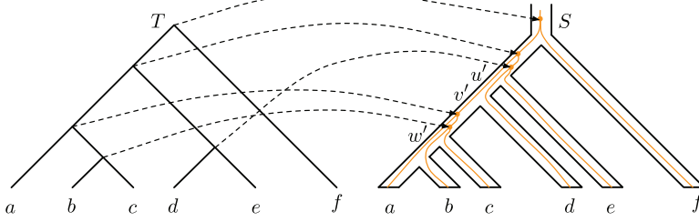
FIG. 1. Computing the deep coalescence cost. Gene tree T is fitted onto species tree S according to a most recent common ancestor (MRCA) mapping. In the figure, mappings between leaves are omitted, and for clearer illustration of how T is reconciled within S , the MRCAs of the internal nodes of T are placed along the branches of S
