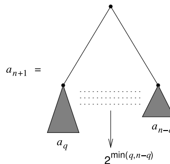
Fig. 6. Decomposition of an ordered ranked tree of size n + 1 that is in \mathcal{R}_{n+1}^{(mp)} and has no non-maximally probable subtrees. The two subtrees of the root are taken from \mathcal{R}^{(mp)} , with sizes q and n - q . According to the definition of maximally probable subtrees, once names L and R are assigned to the two subtrees in such a way that |R| = \min(q, n - q) , the number of possible rankings to obtain a sequence of coalescences satisfying (3) is 2^{|R|} .
