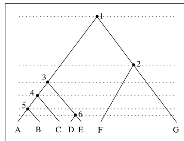
Fig. 2. A ranked species tree that is non-maximally probable at internal node 3. This tree is maximally probable at the root.
